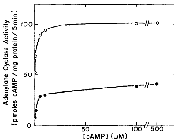
Fig.1. Activation of adenylate cyclase by cAMP. Assays were carried out as described in the text. The effect of cAMP was studied on adenylate cyclase in the particulate fraction (○) and in the supernatant fraction (●).
